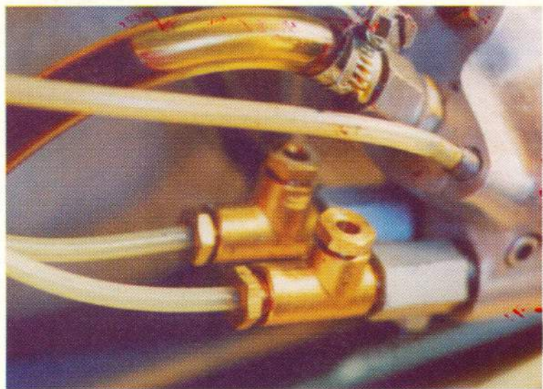
Ged Rumble's 'air-bleed' units to overcome crank-case suction — described in an earlier Yowl .
