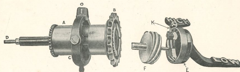
Gear Hub Assembly with Driving Sprocket.
