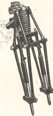
The Scott Girder Forks as fitted to Flying Squirrel De Luxe and T.T. Replica.
