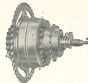
The Complete Gear Assembly.
