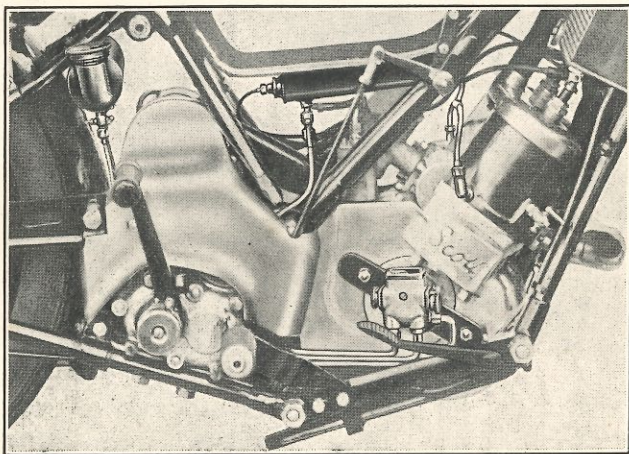
Showing Lubrication Details of Power-plus T.T. Replica.
