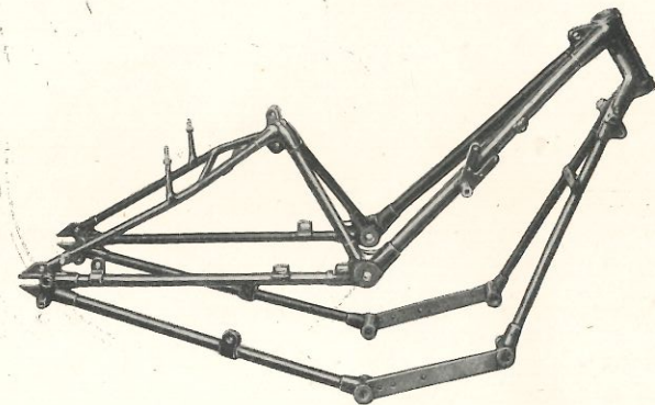
The Scott Frame—Flying Squirrel Type. The top-tube (not shown) carries the petrol tank and is readily detachable.
